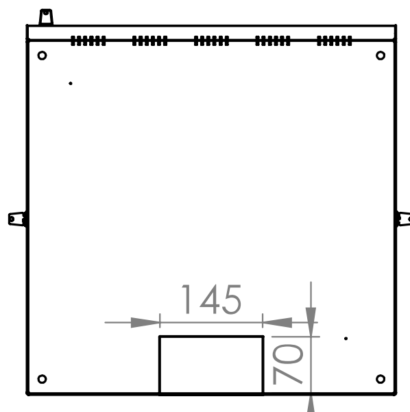
Bottom view
