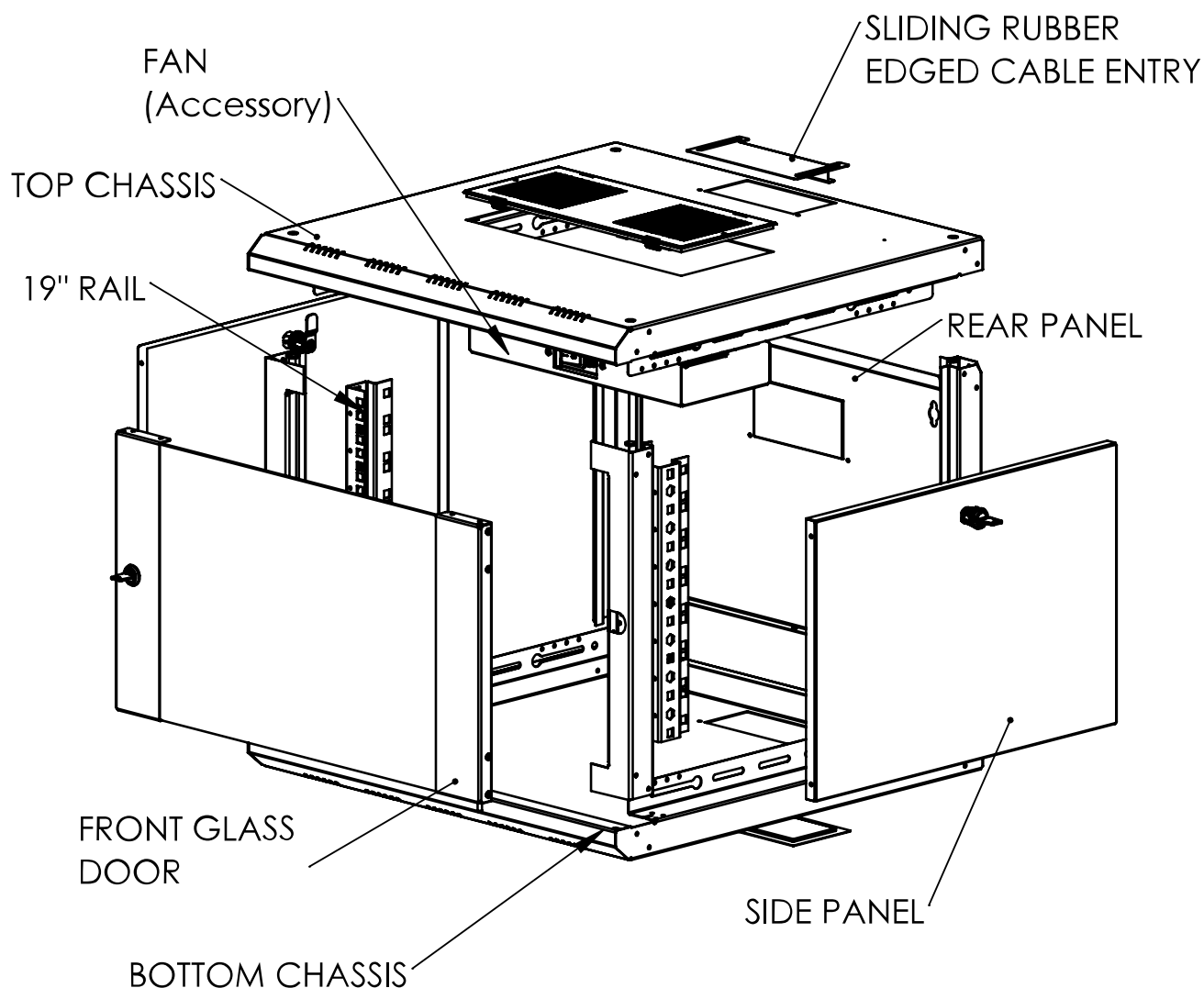
Exploded view
